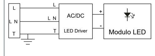
CARACTERÍSTICAS DEL DRIVER LED X6-105M150
